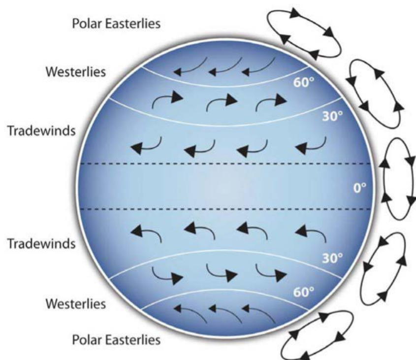
Figure 9.1 - Coriolis Effect
